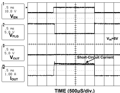
Enabled Into Short (AP1212H)
