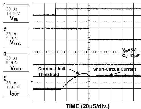
Current-Limit Response (AP1212H)
