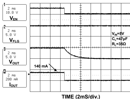
Turn-Off (AP1212H)
