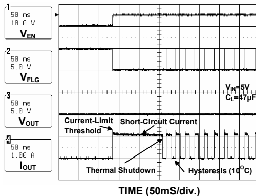
Current-Limit Response (AP1212H)
