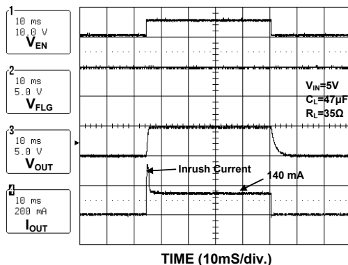
Turn-On/Turn-Off (AP1212H)
