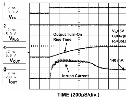
Turn-On (AP1212H)
