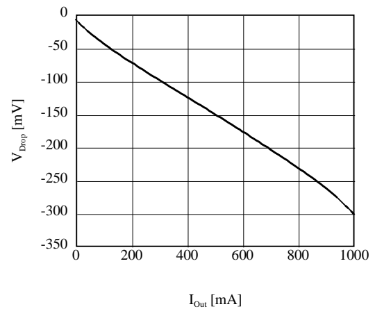
■ V_{\text{Drop}} vs I_{\text{Out}} (AP1155ADU)
