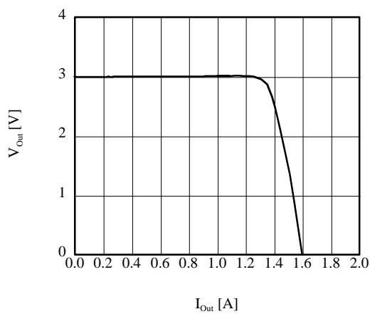
■ V_{\text{Out}} vs I_{\text{Out}} (AP1155ADU)
