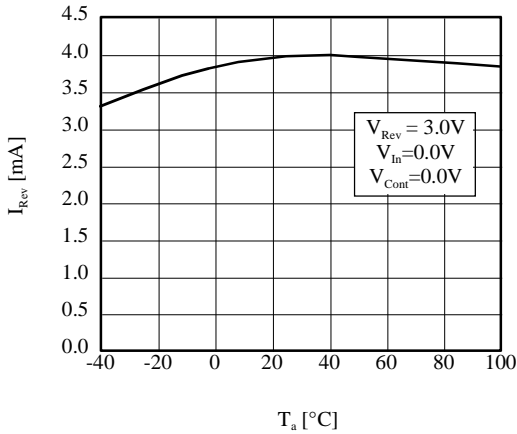
■ Reverse Bias Current( I_{\text{Rev}} ) vs T_a (AP1155ADU)
