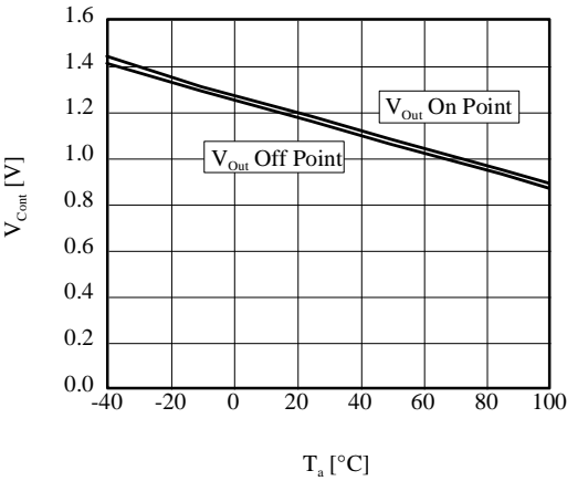
■ V_{\text{Out}} On/Off Point vs T_a (AP1155ADU)
