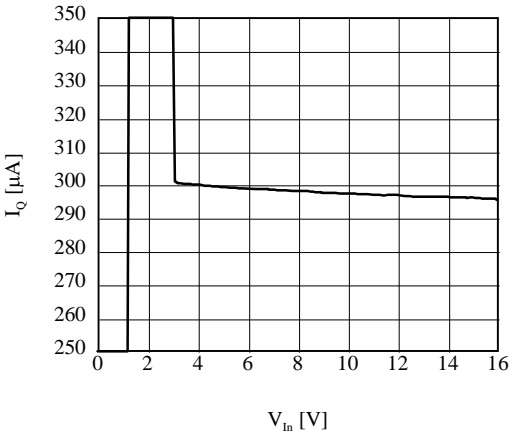
■ I_{\text{Q}} vs V_{\text{In}} (AP1155ADU)
