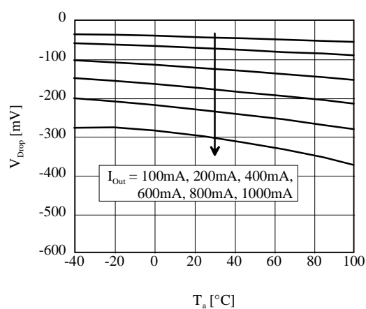
■ V_{\text{Drop}} vs T_a (AP1155ADU)
