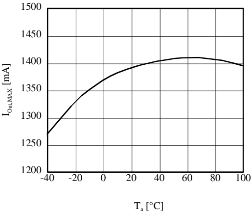
■ I_{\text{Out,MAX}} vs T_a (AP1155ADU)
