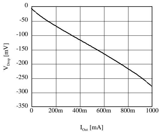
■ V_{\text{Drop}} vs I_{\text{Out}} (AP1155ADU)
