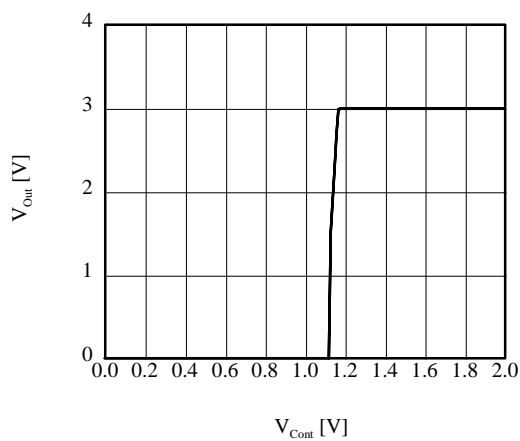
■ V_{\text{Out}} vs V_{\text{Cont}} (AP1155ADU)
