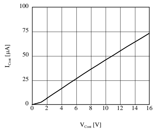
■ I_{\text{Cont}} vs V_{\text{Cont}} (AP1155ADU)
