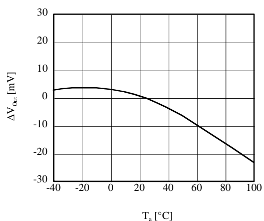
■ \Delta V_{\text{Out}} vs T_a (AP1155ADU)
