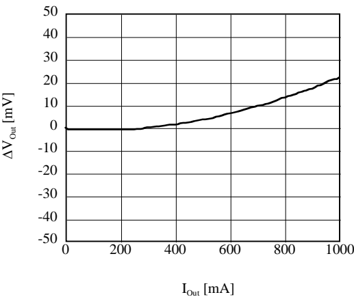
■ \Delta V_{\text{Out}} vs I_{\text{Out}} (AP1155ADU)
