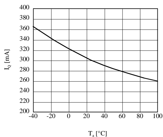
■ I_Q vs T_a (AP1155ADU)
