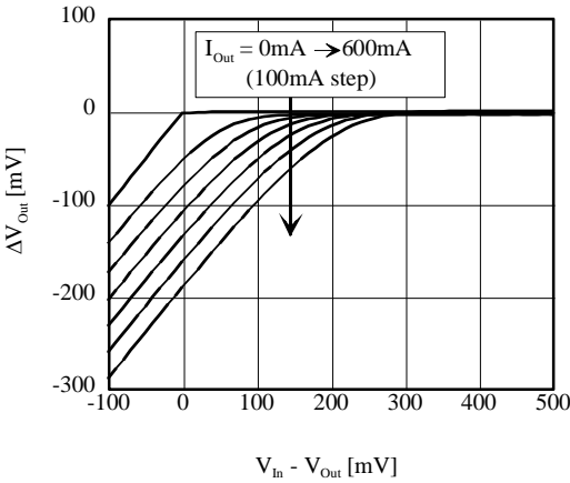
■ \Delta V_{\text{Out}} vs V_{\text{In}} (AP1155ADU)
