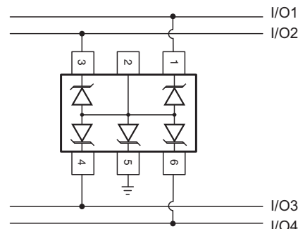
Bidirection Protection of Four Lines
