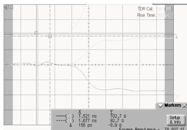
Figure 14. 140Ω Differential Impedance with Package on it Max. 102Ω, Min. 92Ω
