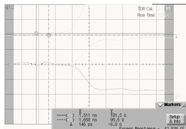
Figure 15. 160Ω Differential Impedance with Package on it Max. 101Ω, Min. 95Ω
