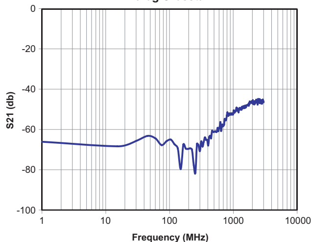
Analog Crosstalk
