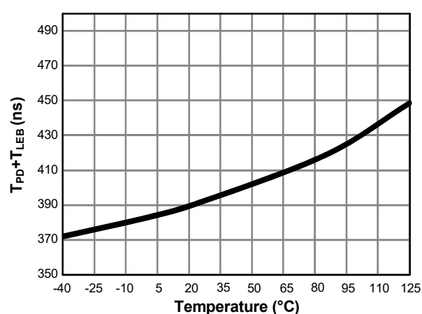
Figure 6. Minimum of the Turn-on Period vs. Temperature
