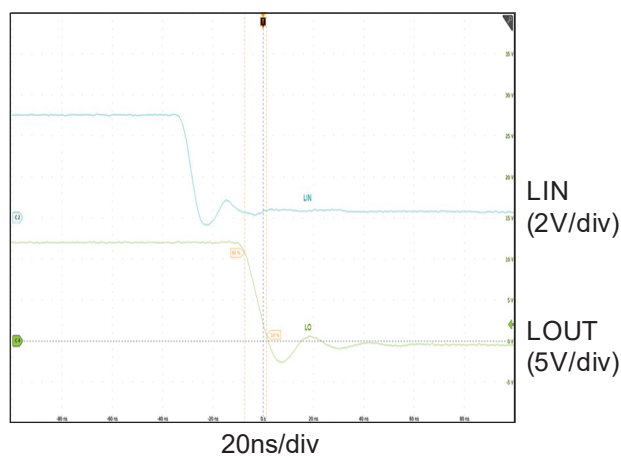
LOUT Fall Time = 8.63ns
