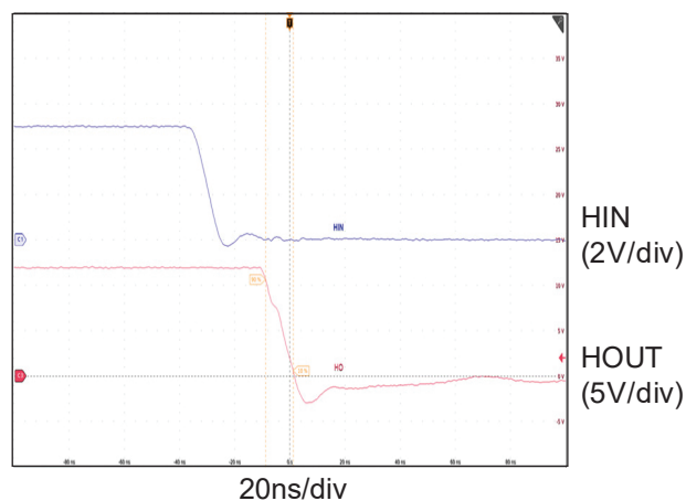
HOUT Fall Time = 10ns
