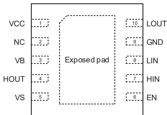
Figure 1. DFN3x3-10L (Top Transparent View)
