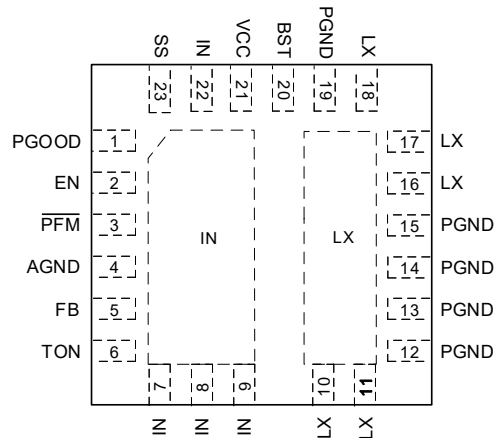
AOZ2263BQI-18 23-Pin 4mm x 4mm QFN
