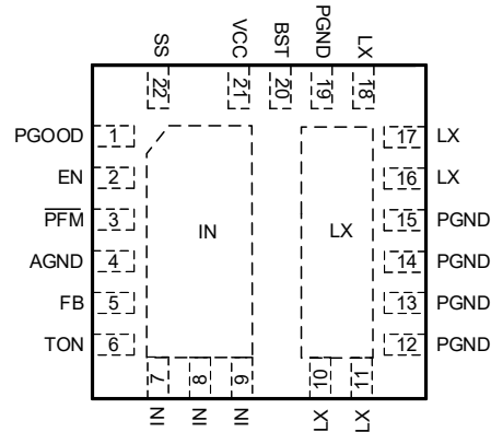
AOZ2260BQI-10 22-pin 4mm x 4mm QFN
