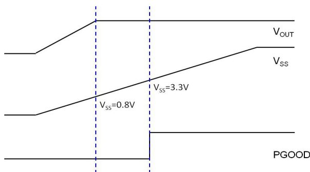
Figure 1. Soft Start Sequence of AOZ2260BQI-10
