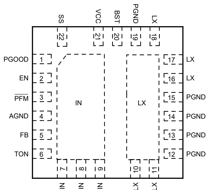
AOZ22421QI 4mmx4mm QFN-22L
