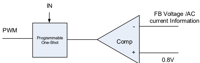
Figure 3. Simplified Control Schematic of AOZ22421QI
