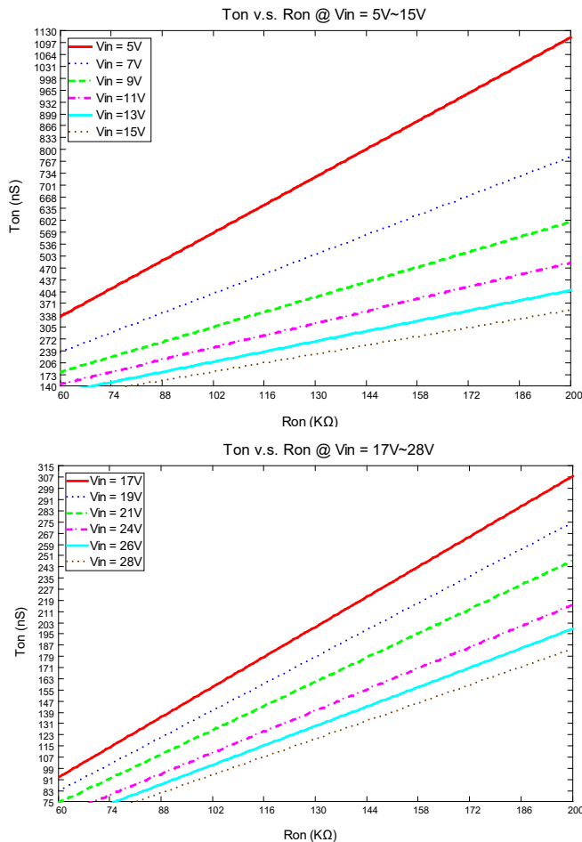
Figure 4. Ton vs. Ron Curves for AOZ22421QI
