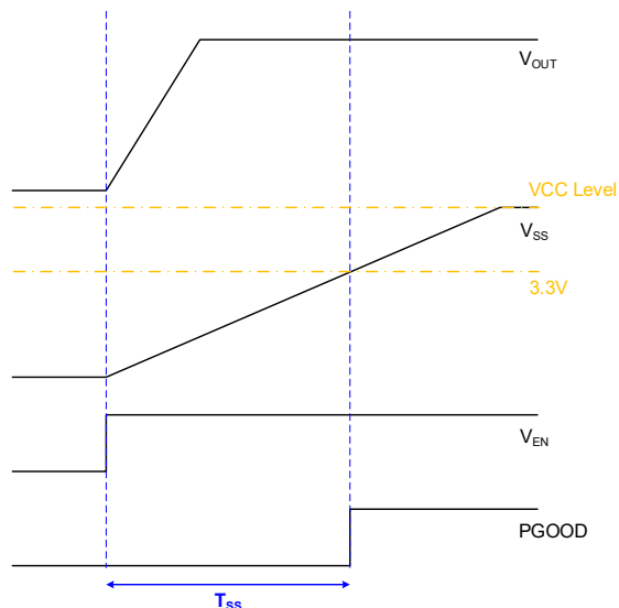
Figure 2. Soft Start Sequence of AOZ22421QI
