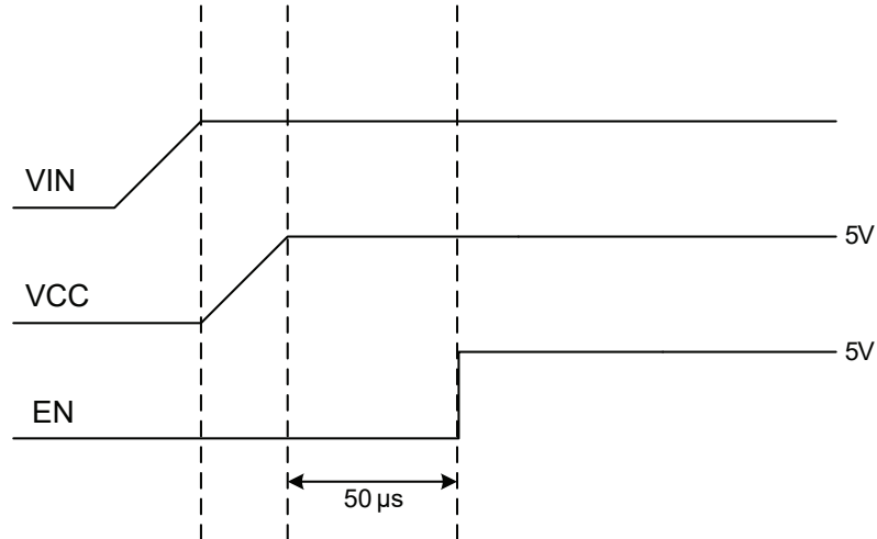
Figure 1. Start-up Sequence
