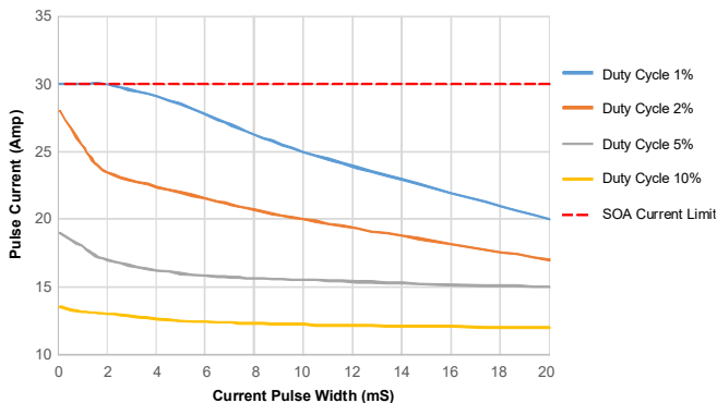
Figure 11. AOZ13986DI-02 Sinking Switch Pulsed Current vs. Duration for a Given Duty Cycle
