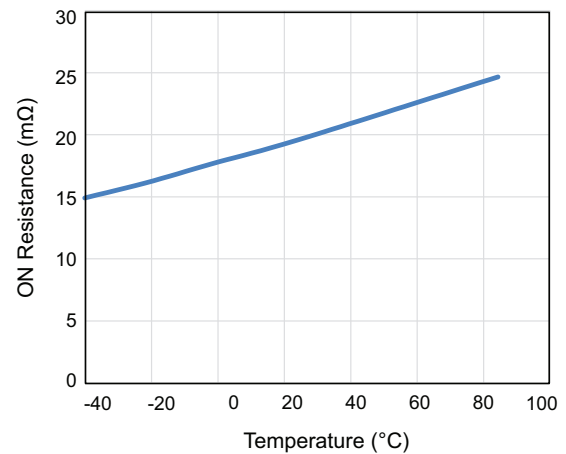
Figure 6. ON Resistance vs. Temperature ( V_{IN}=20\text{V} )
