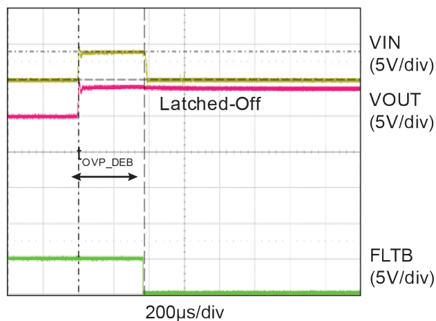
Over-Voltage Protection
