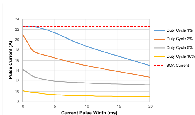
Figure 11. AOZ13984DI-01 Sinking Switch Pulsed Current vs. Duration for a Given Duty Cycle
