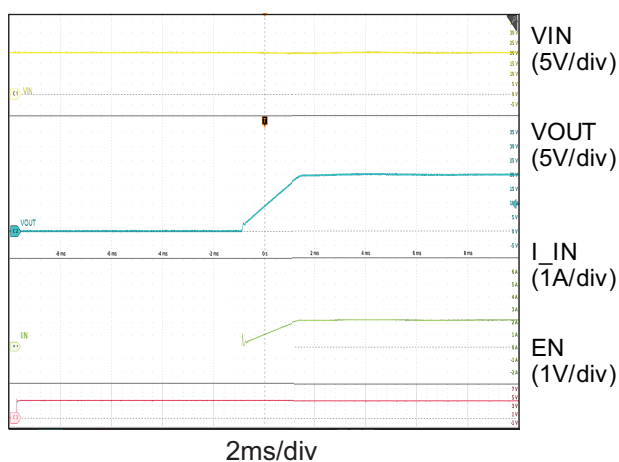
Soft-Start Ramp ( V_{IN} = 20\text{V} , R_{OUT} = 9.06\Omega )
