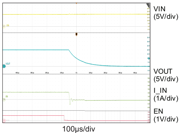
Shutdown ( V_{IN} = 20\text{V} , R_{OUT} = 9.06\Omega )
