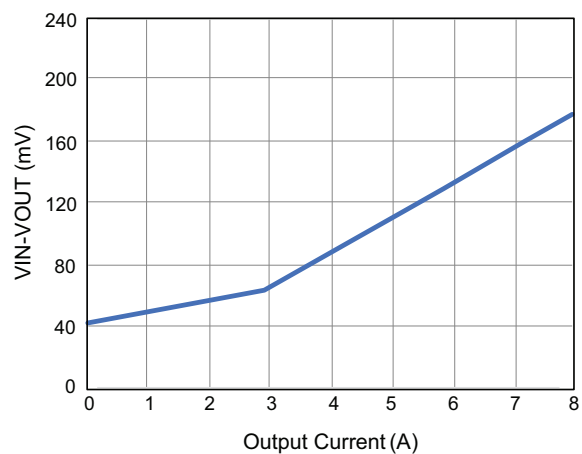
Figure 8. VIN-VOUT vs. Output Current
