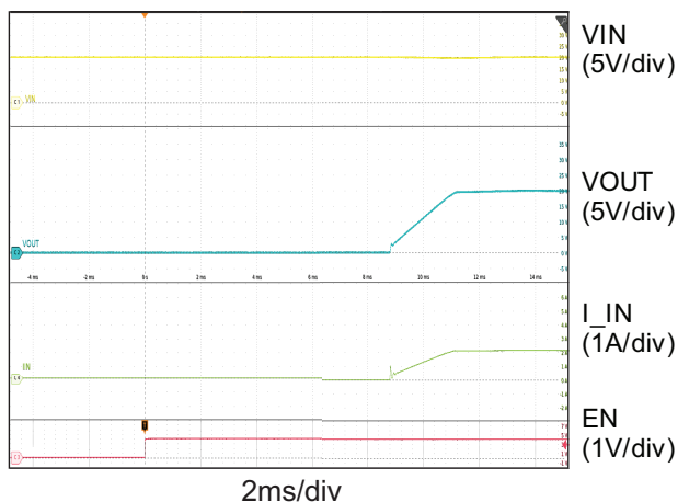
Soft-Start Delay ( V_{IN} = 20\text{V} , R_{OUT} = 9.06\Omega )
