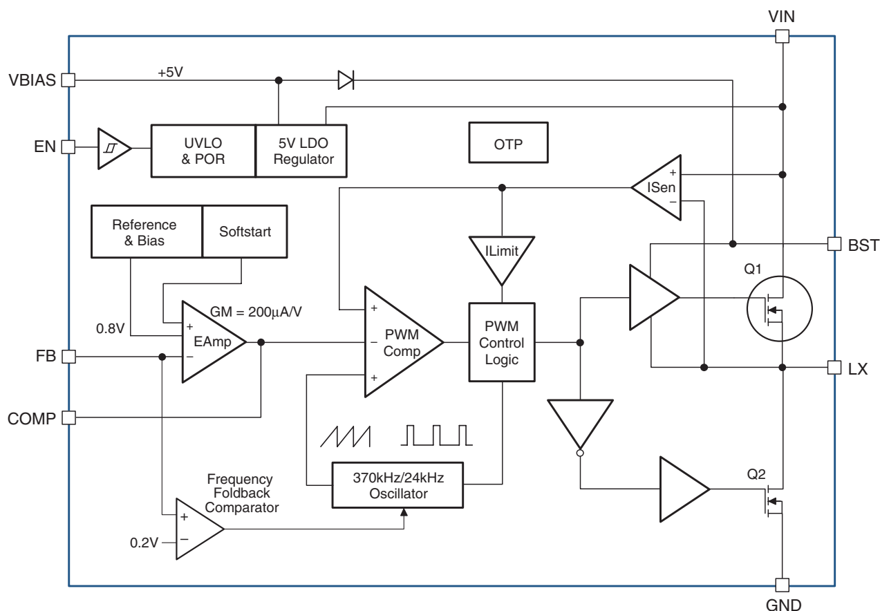
Block Diagram
