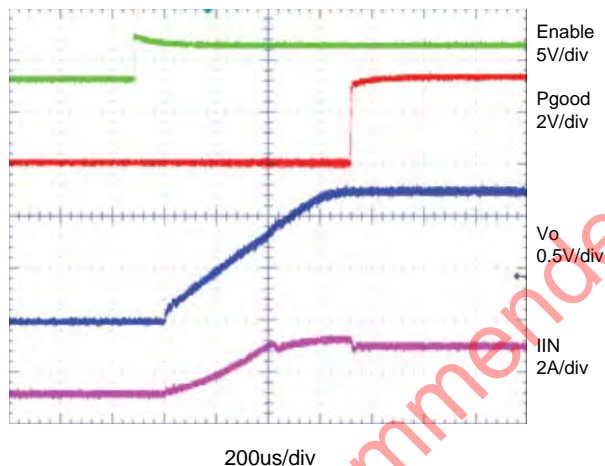
Start Up Waveforms
