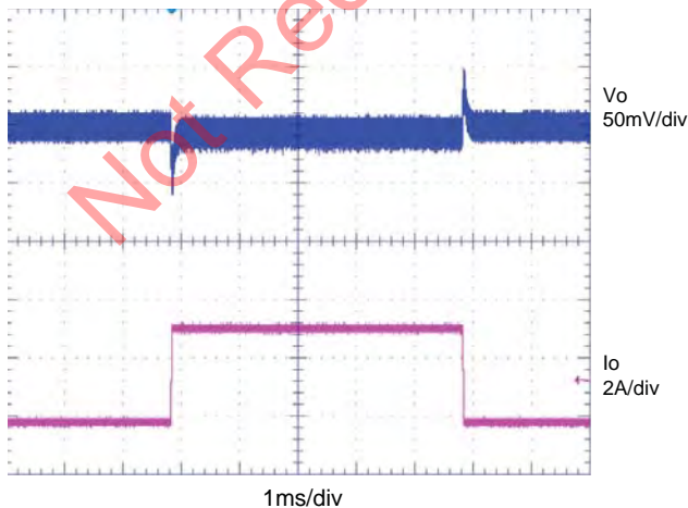
Load Transient Waveforms
