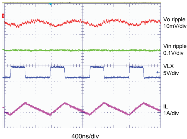
Switching Waveforms at Light Load
