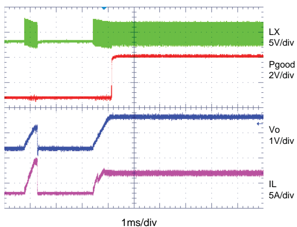
Short-Circuit Recovery Waveforms
