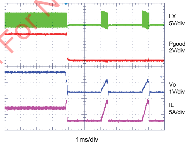
Short-Circuit Protection Waveforms
