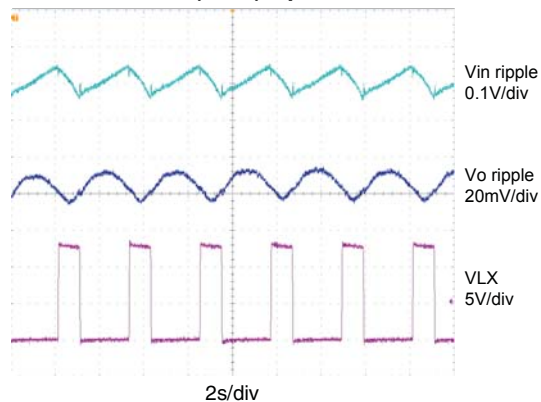
Full Load (CCM) Operation
