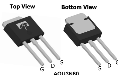
TO251
