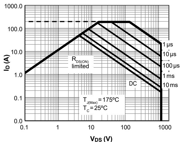
Figure 17. Maximum Forward Biased Safe Operating Area for AOM033V120X3Q (Note K)
