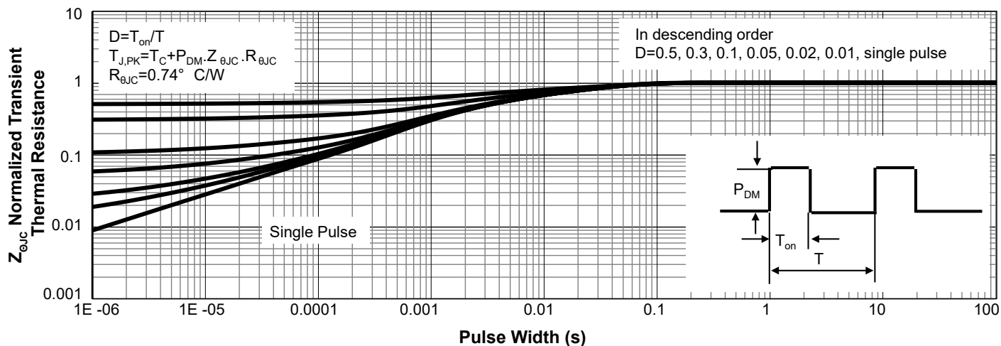
Figure 18. Normalized Maximum Transient Thermal Impedance for AOM033V120X3Q (Note K)
