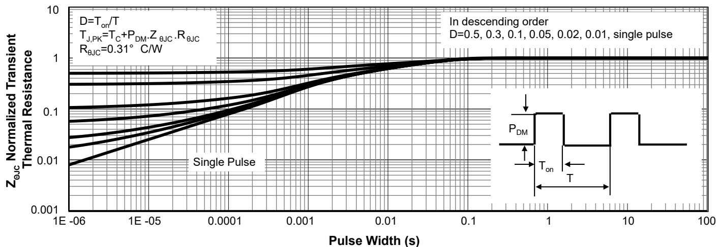
Figure 18. Normalized Maximum Transient Thermal Impedance for AOM020V120X3Q (Note K)
