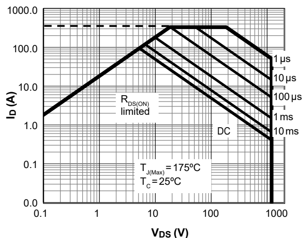
Figure 17. Maximum Forward Biased Safe Operating Area for AOM020V120X3Q (Note K)
