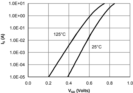
Figure 6: Body-Diode Characteristics
