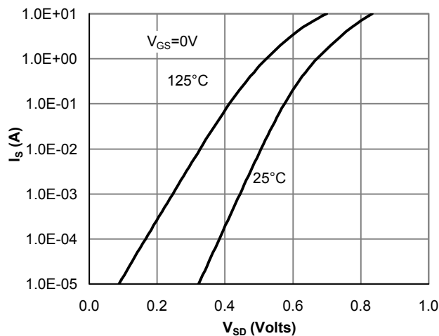
Figure 6: Body-Diode Characteristics
