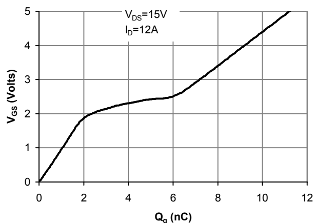
Figure 7: Gate-Charge Characteristics
