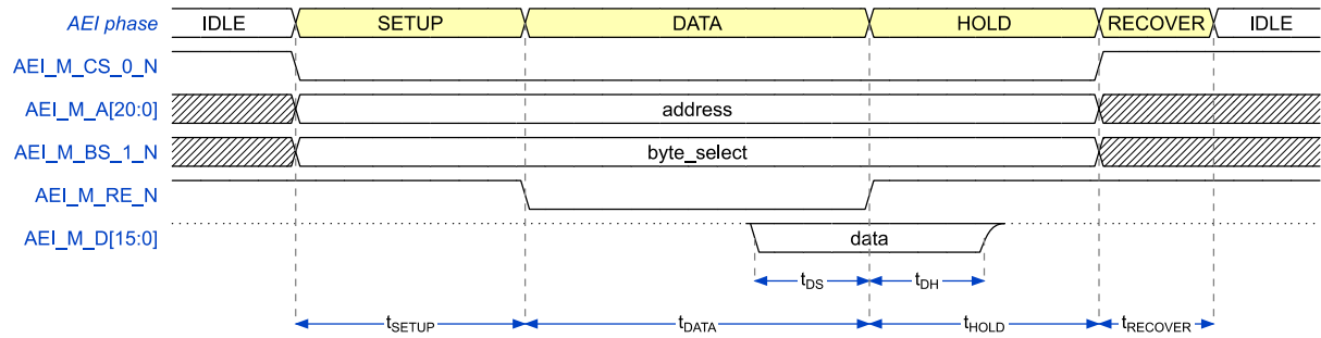
Figure 8-4 AEI Master – Read Transfer (Wait Signal Used)
