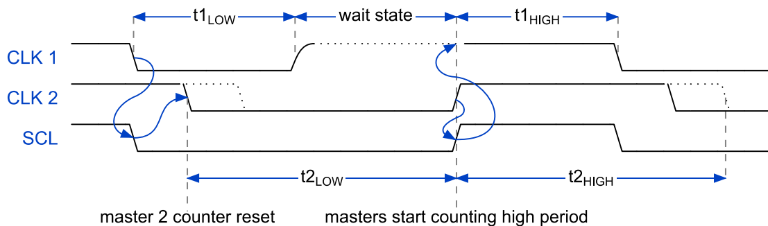
Figure 8-28 I 2 C – clock synchronization
