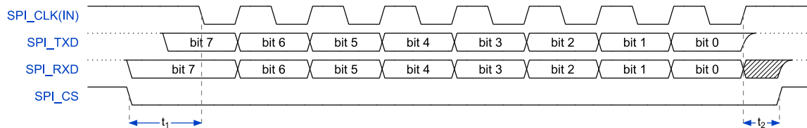
Figure 8-22 SPI – Transfer Format Mode 3
