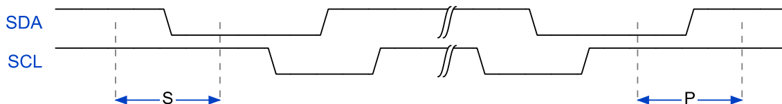
Figure 8-26 I 2 C – START and STOP conditions
