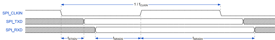
Figure 8-24 SPI – Slave Mode Timing
