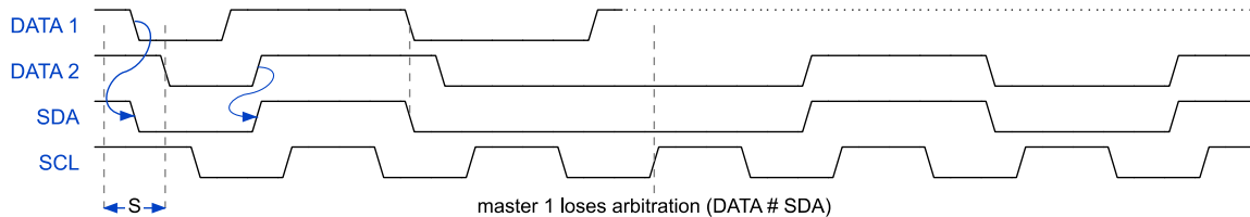
Figure 8-29 I 2 C – Arbitration
