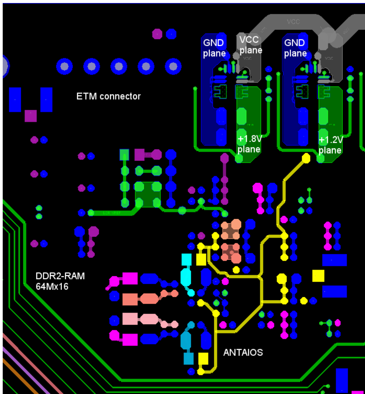
Figure 9-6 Bottom Layer
