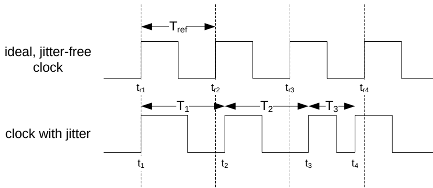
Figure 7-4 Jitter Definition
