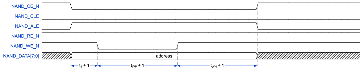
Figure 8-11 NAND Flash – Write Data Timing
