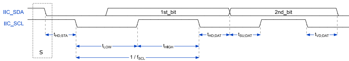
Figure 8-31 I 2 C – Input/Output Timing (2)
