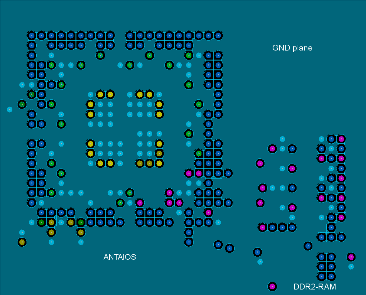
Figure 9-8 Internal Layer 1
