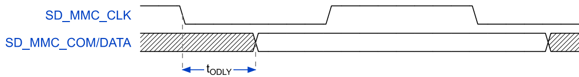
Figure 8-16 SD/MMC –Output Timing (ID Mode; Data Transfer – Default Speed)
