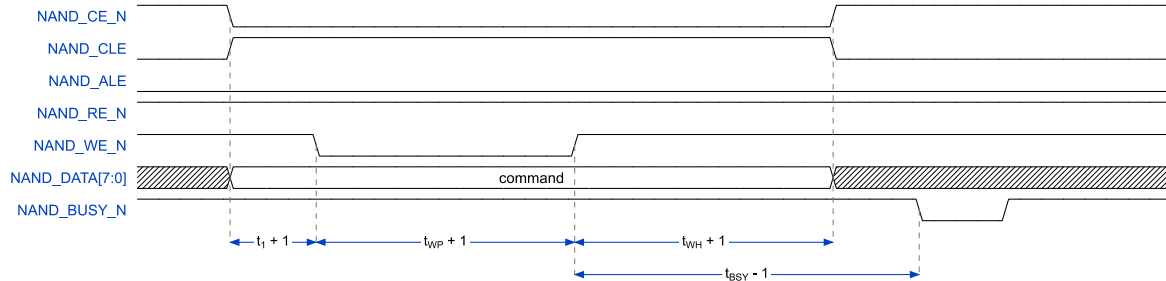
Figure 8-10 NAND Flash – Address Latch Timing
