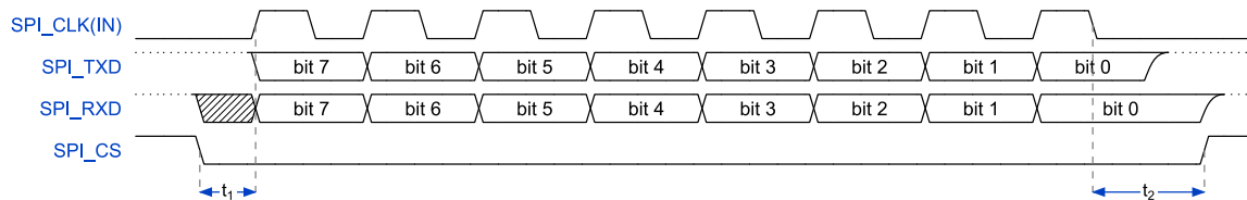
Figure 8-21 SPI – Transfer Format Mode 2
