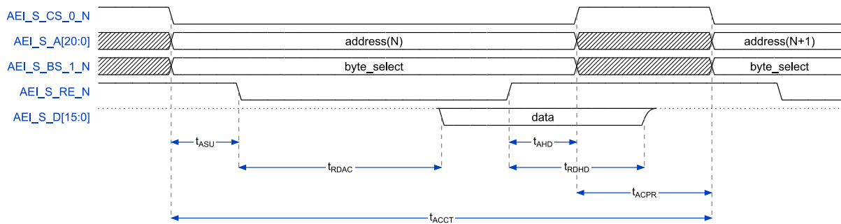
Figure 8-8 AEI Slave – Read Transfer (Wait Signal Used)
