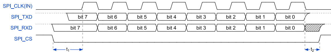
Figure 8-20 SPI – Transfer Format Mode 1
