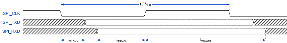
Figure 8-23 SPI – Master Mode Timing
