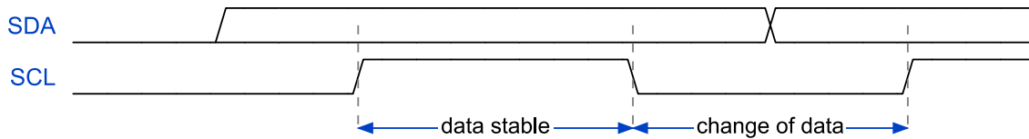
Figure 8-25 I 2 C – Bit Transfer
