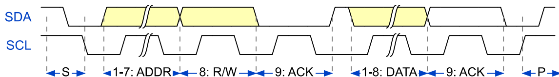
Figure 8-27 I 2 C – Data Transfer
