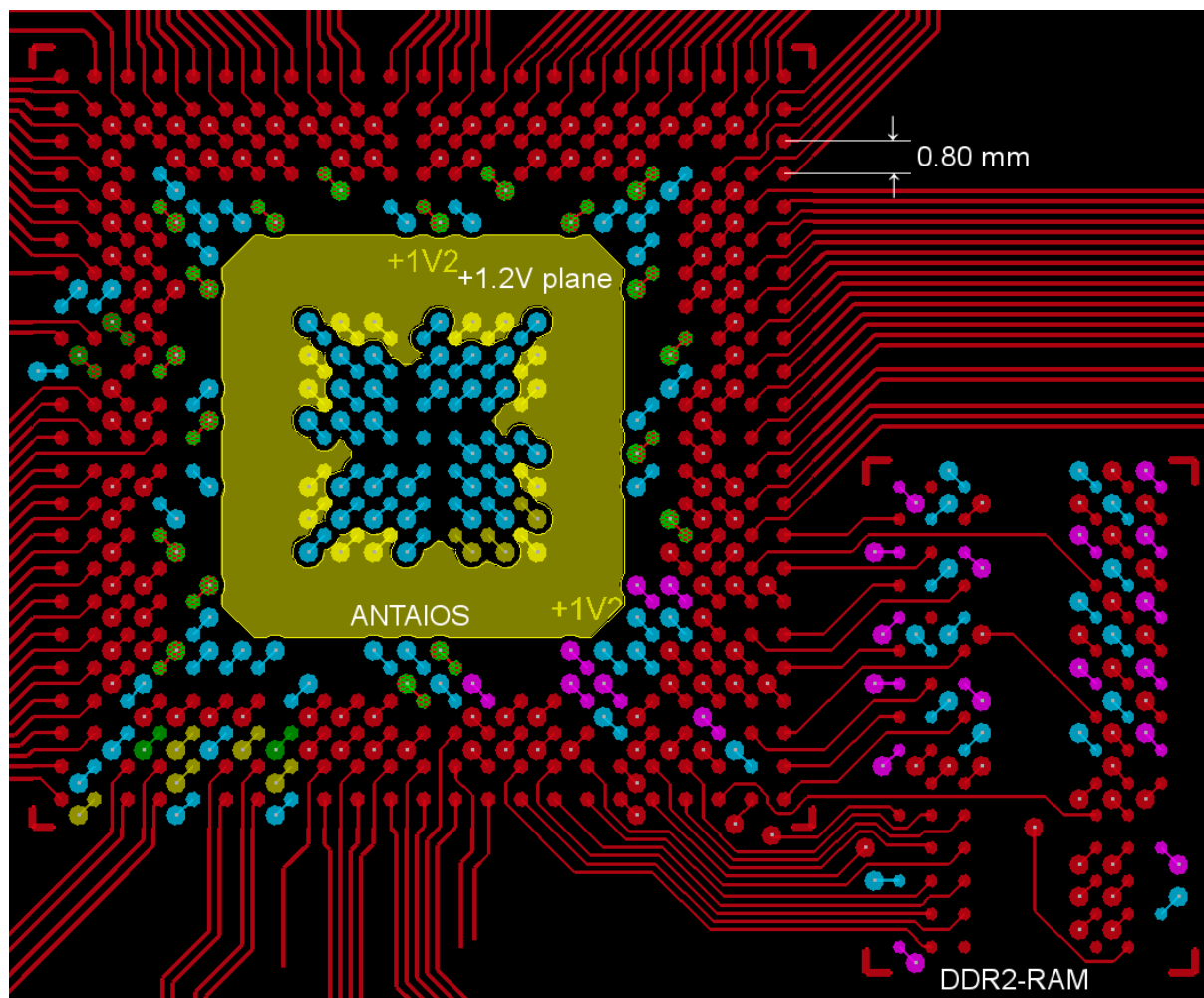
Figure 9-7 Top Layer
