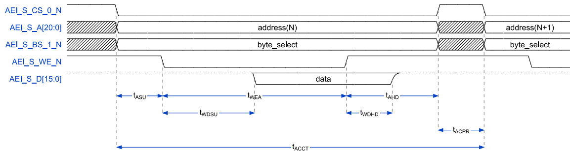
Figure 8-6 AEI Slave – Write Transfer (Wait Signal Used)
