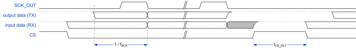
Figure 8-14 QSPI – Setup and Hold Timing
