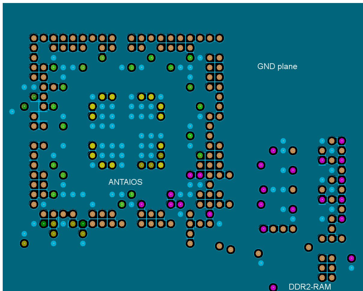
Figure 9-11 Internal Layer 4
