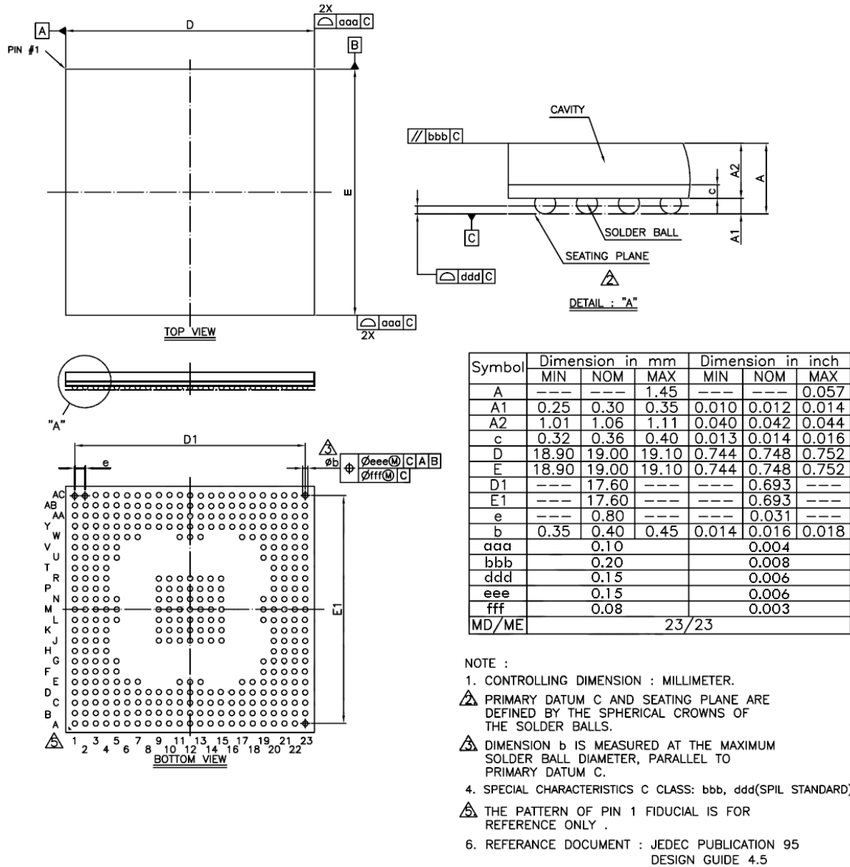
Figure 10-2 TFBGA-385 Package Dimensions and Tolerances
