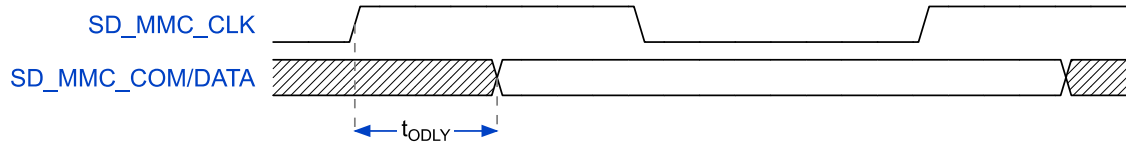
Figure 8-18 SD/MMC –Input Timing
