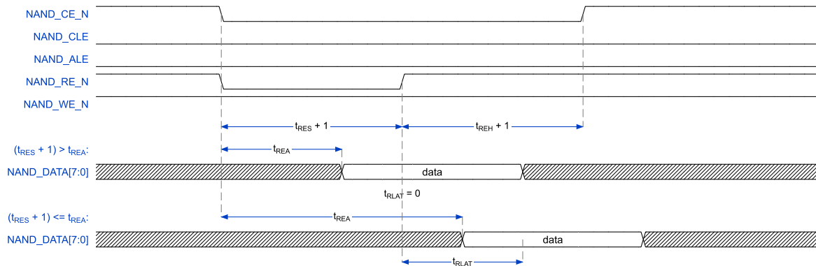
Figure 8-12 NAND Flash – Read Data Timing
