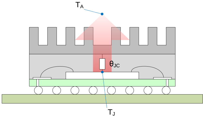
Figure 7-3 Heat Flow (with heat sink)
