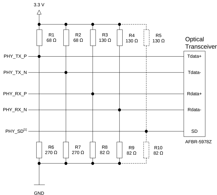
Figure 4-3 Optical Interface
