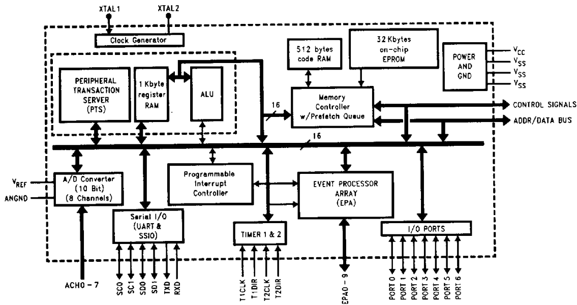
87C196KT Block Diagram
