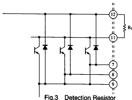
Fig.3 Detection Resistor
