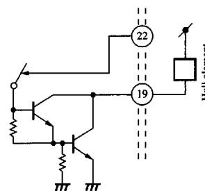
Fig.8 Hall Switch
