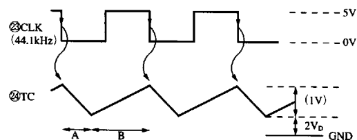
Fig.4 Saw-tooth Wave Generator
