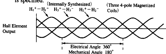
Fig.1 Output and Hall Element Output
