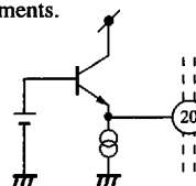
Fig.9 Hall Bias
