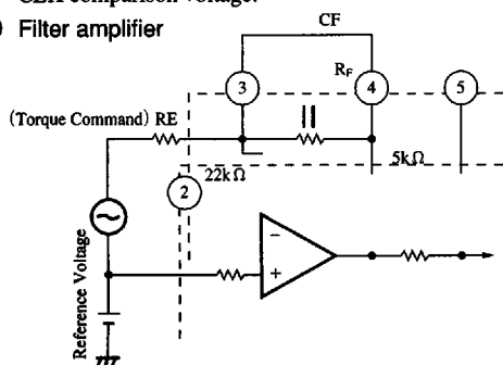
Fig.6 Ripple Filter
