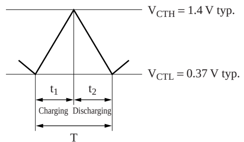
Figure 3. Triangular wave oscillation waveform
