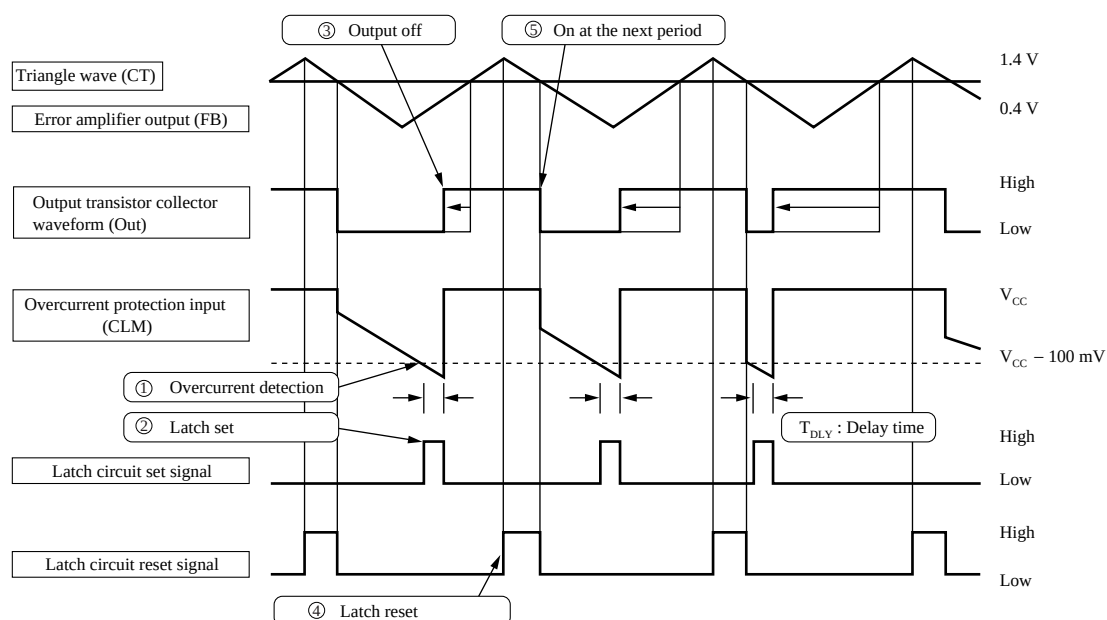
Figure 2. Pulse-by-pulse overcurrent protection operating waveforms
