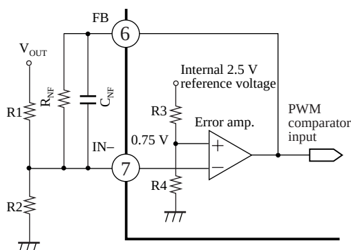
Figure 1. Connection method of error amplifier
