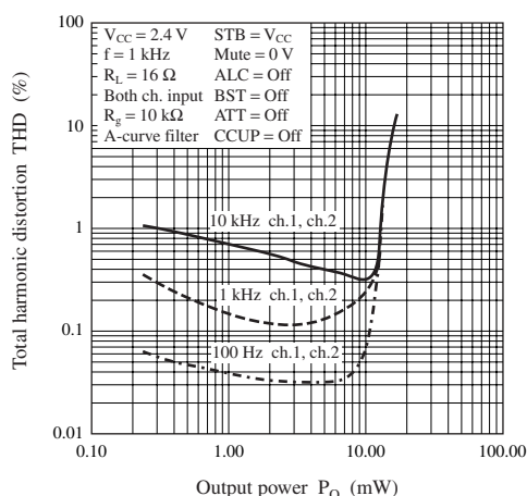
\text{THD} - P_O
