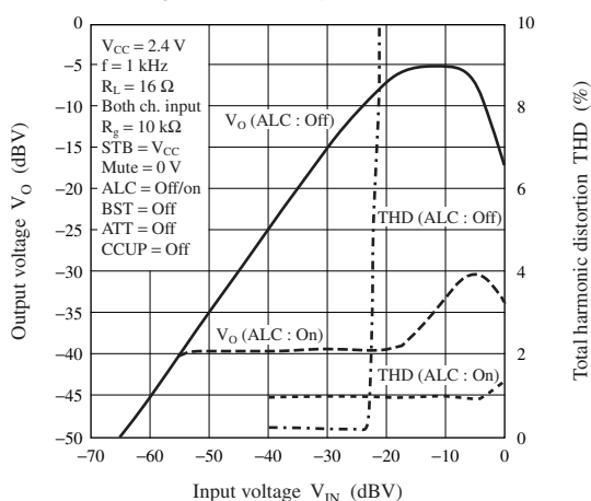
P_O, \text{THD} - V_{IN} (\text{ALC: On})
