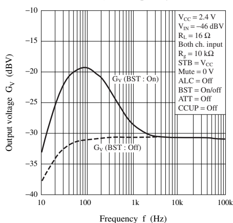
G_V - \text{frequency}
