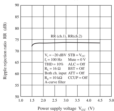
RR — V_{CC}
