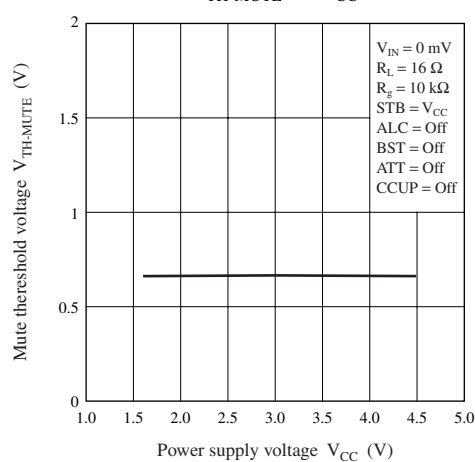
V_{TH-MUTE} — V_{CC}
