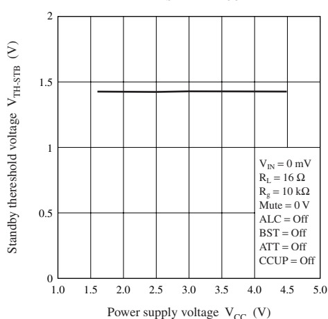
V_{TH-STB} — V_{CC}
