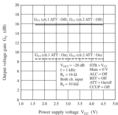
G_V - V_{CC}
