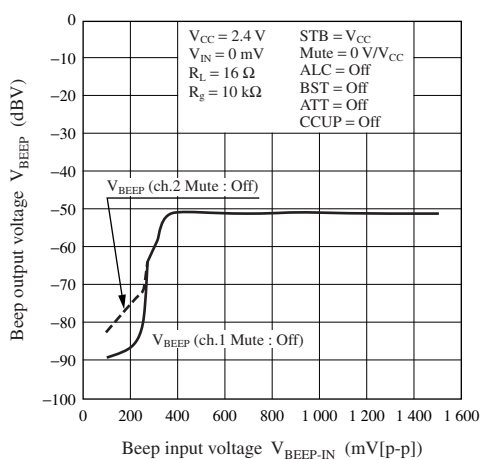
\text{Beep} - V_{IN}
