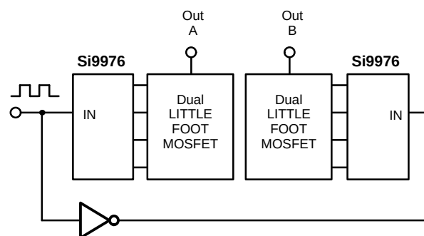
Figure 5. Anti-Phase Control
