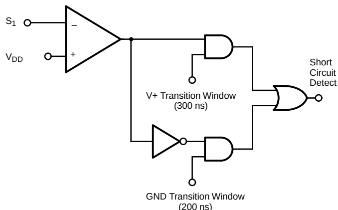
Figure 4. Short Circuit Protection
