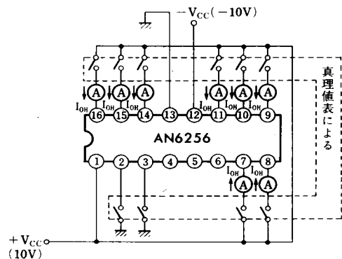
Test Circuit 3 ( I_{OH(2)} )
