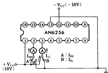
Test Circuit 1 ( I_{IH} , -I_{IL} )
