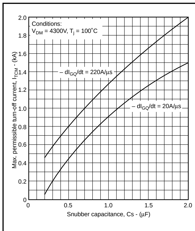
Fig. 6 Max. permissible turn-off current vs snubber capacitance
