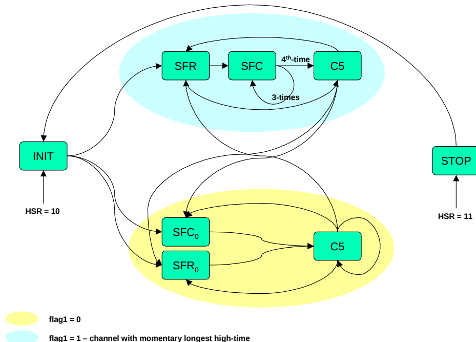
Figure 5. svmStd3Xor_R state diagram
