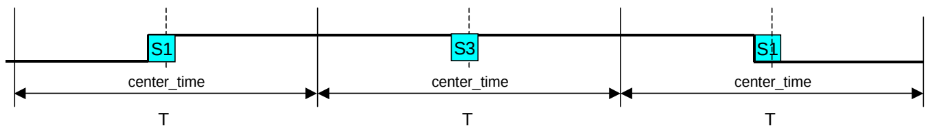
Figure 10. svmStd3Xor_res timing
