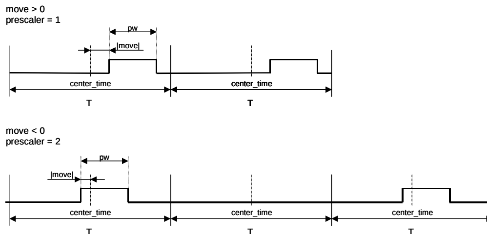
Figure 6. Synchronization signal adjustment examples
