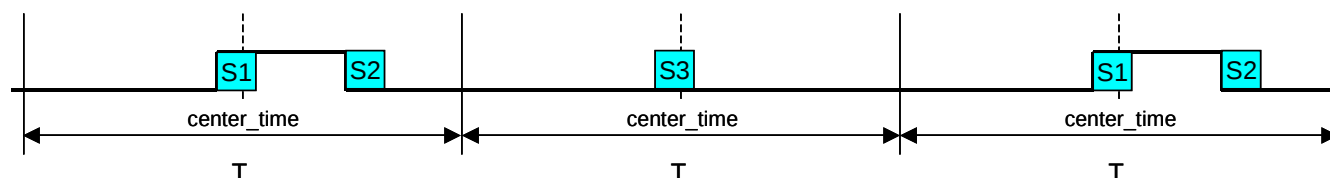
Figure 7. svmStd3Xor_sync timing
