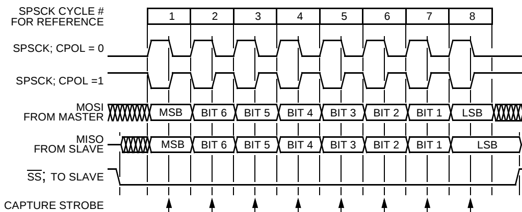
Figure 18. SPI Polarity Chart
