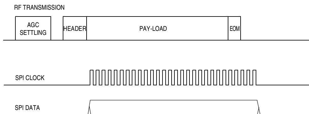
Figure 9. RF Protocol
