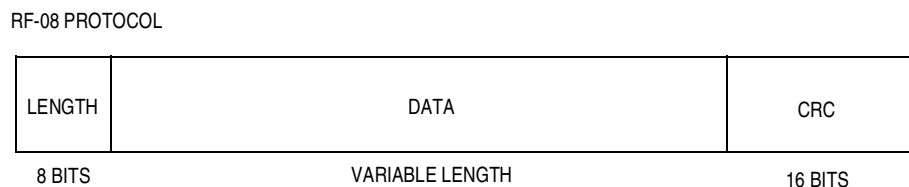
Figure 17. RF-08 Protocol
