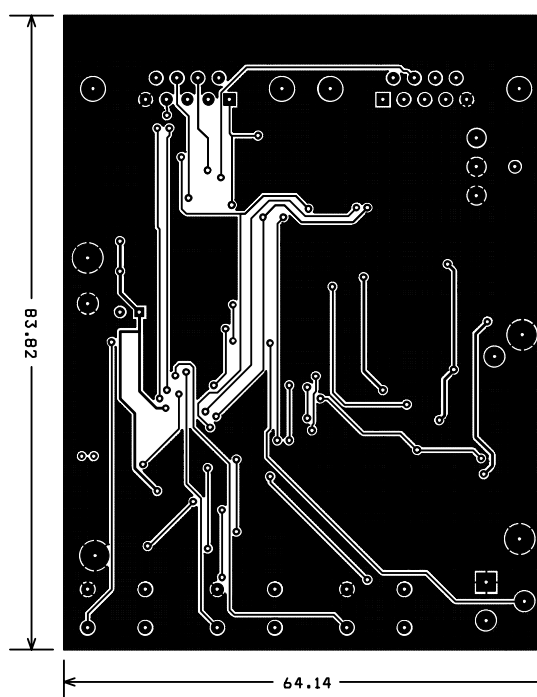
Figure 3. Bottom Copper Side
