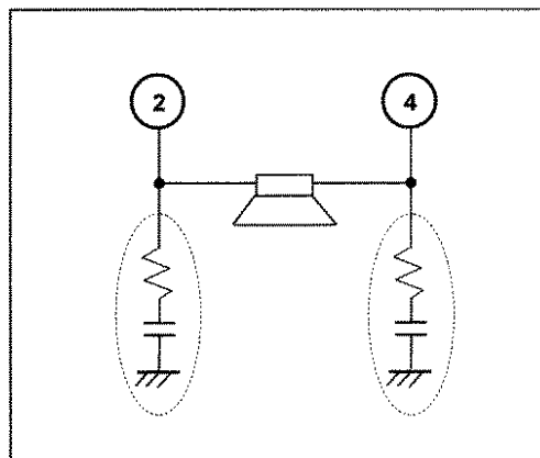
FIG 6. Output Zobel Network
