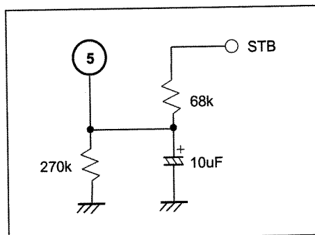
FIG 2. Standby Circuits
