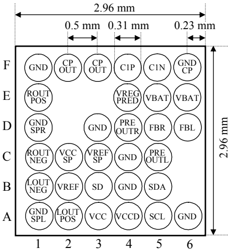
Diagram of pin names on package bottom face
