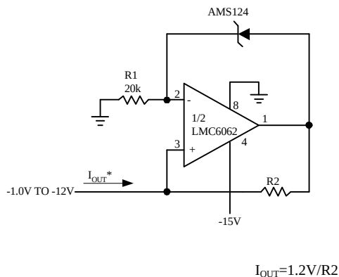
Precision 1 \mu A to 1mA Current Sources
