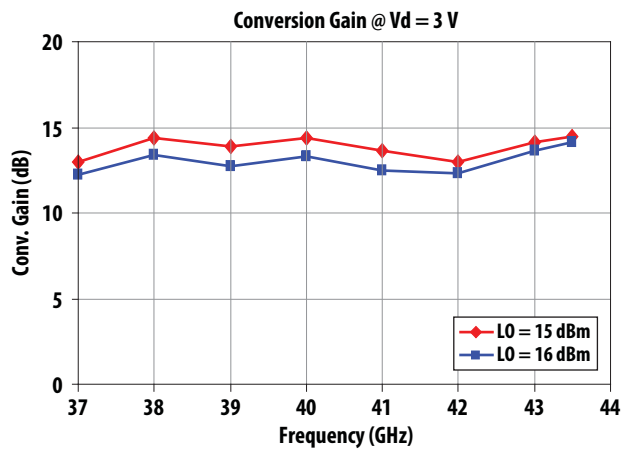
Figure 9. Conversion Gain @ 25° C, Vdd = 3 V, vs. LO Power
