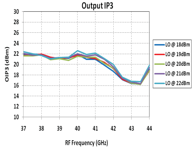
Figure 16. USB Output IP3 vs. RF Freq. @ LO = 18-22 dBm with V_c = -1 V
