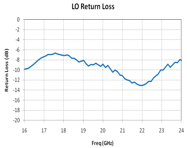
Figure 24. LO Input Return Loss with LO = +20 dBm
