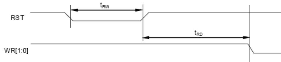
Reset Characteristics
