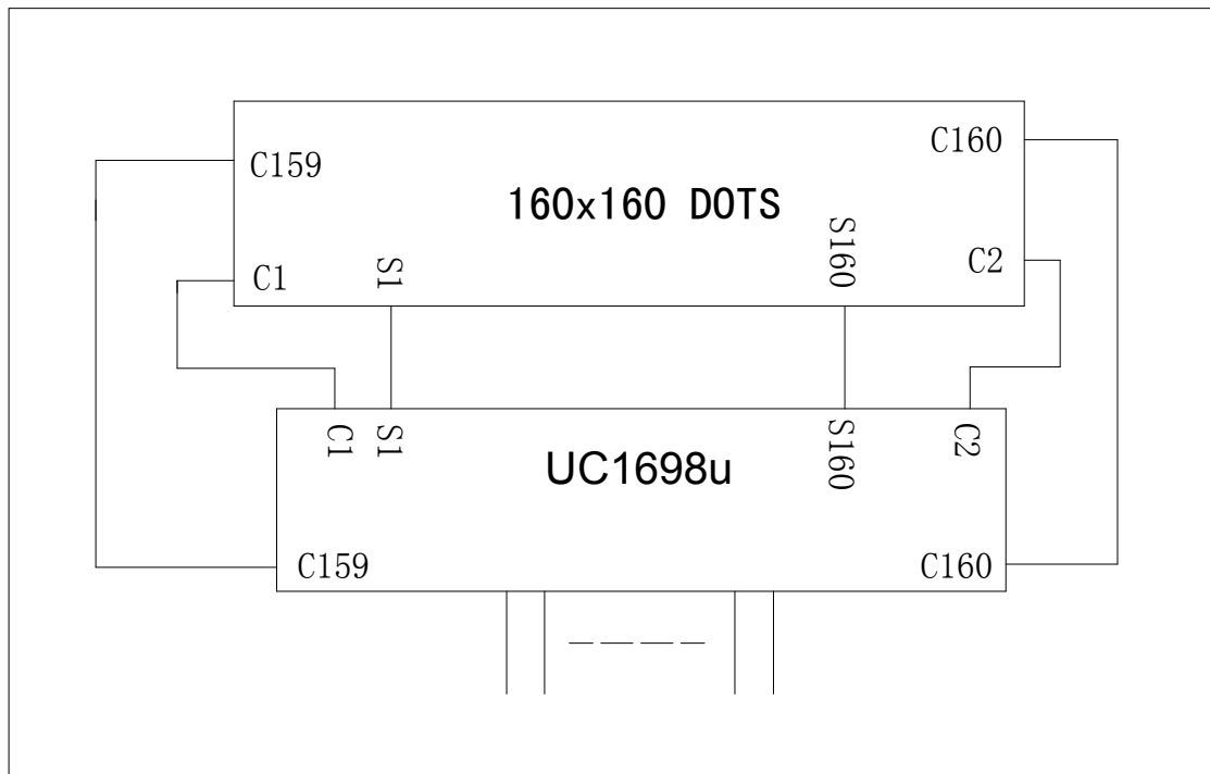
Figure 1. Block diagram
