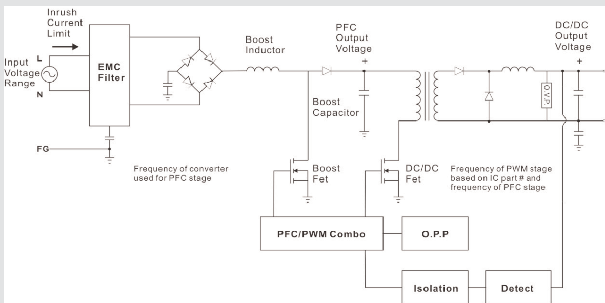
BLOCK DIAGRAM
