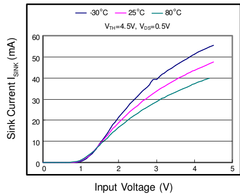
Nch Driver Sink Current vs. Input Voltage
