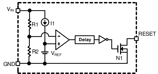
AME8500 with Open-Drain RESET
