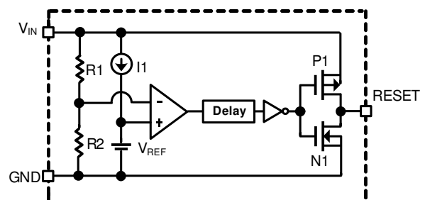
AME8500 with Push-Pull RESET
