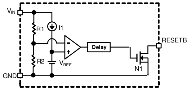
AME8500 with Open-Drain RESETB
