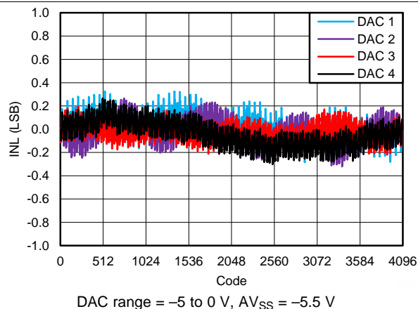
Figure 5. Bipolar DAC Integral Non-Linearity
