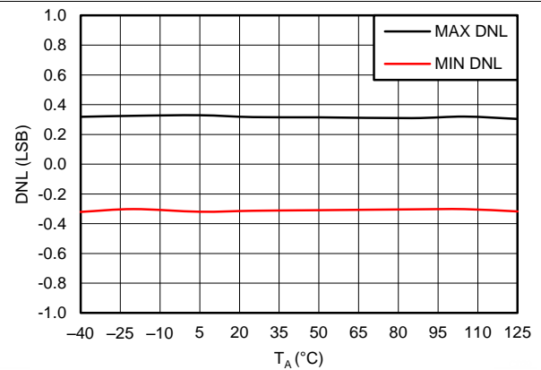
Figure 32. ADC DNL
