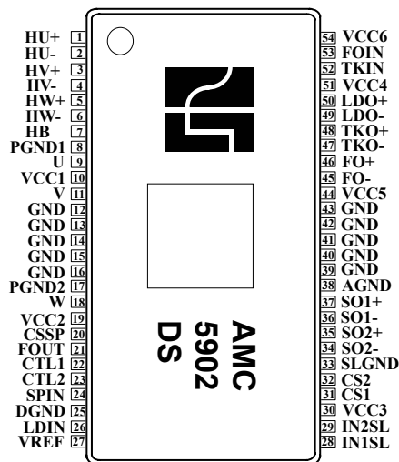
TSOP-54L (TOP VIEW)
