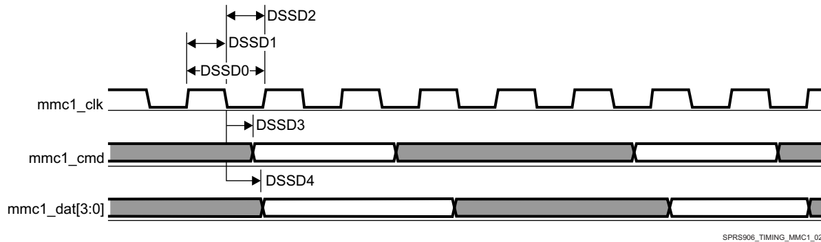
Figure 5-74. MMC/SD/SDIO in - Default Speed - Transmitter Mode
