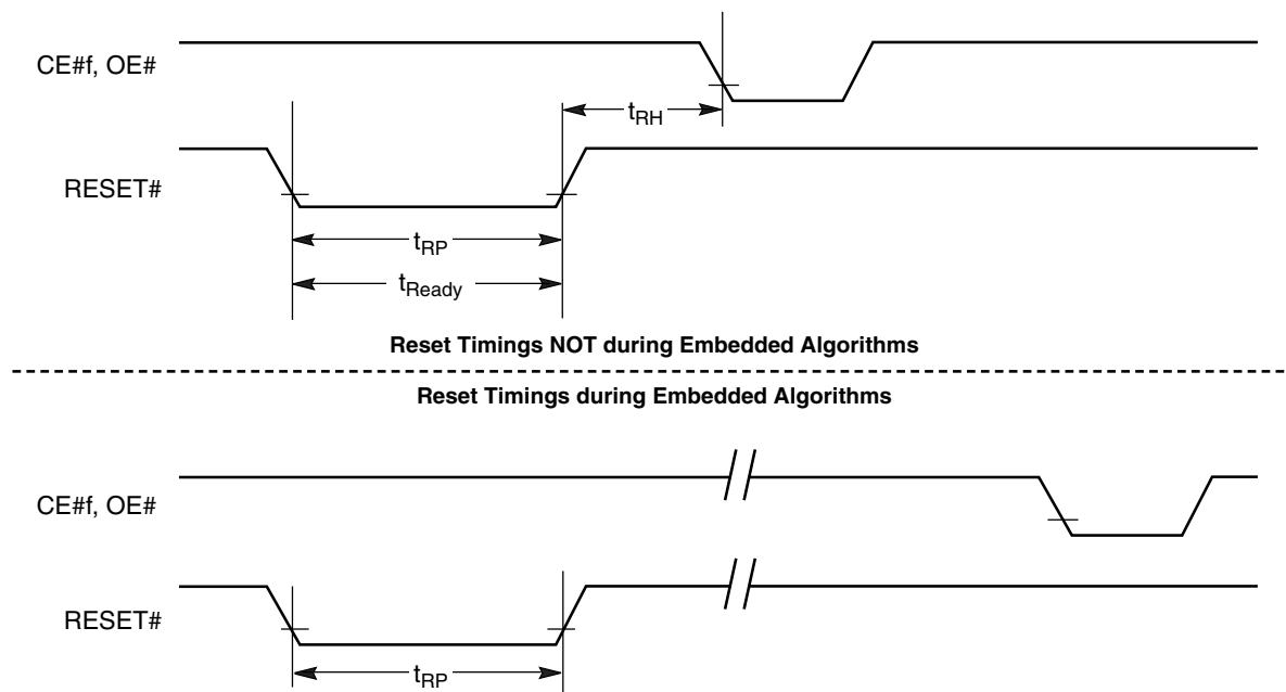
Figure 16. Reset Timings
