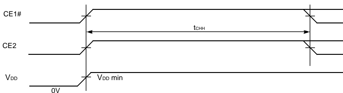
Figure 42. Power-up Timing #1
