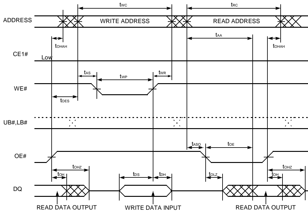
Figure 40. Read/Write Timing #2 (OE#, WE# Control)
