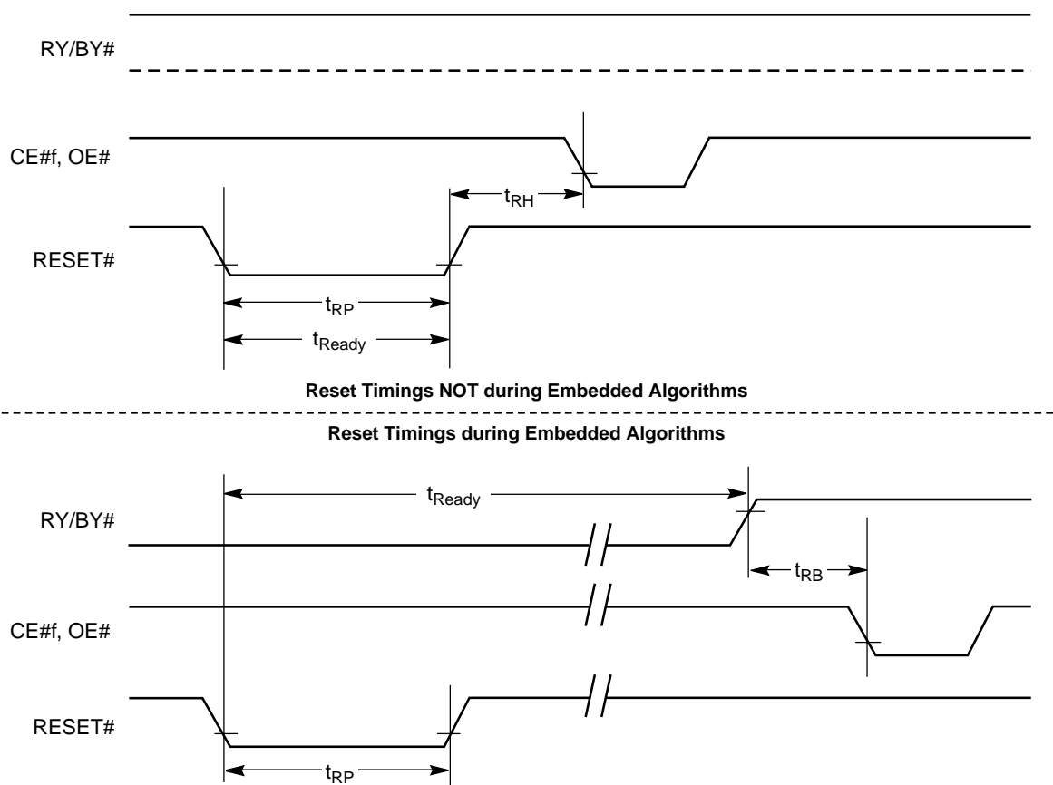
Figure 15. Reset Timings
