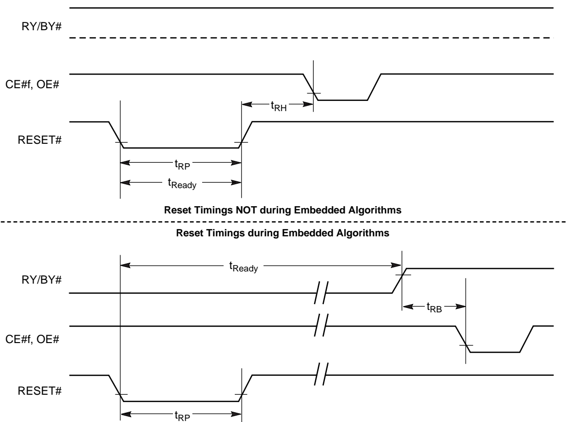
Figure 16. Reset Timings
