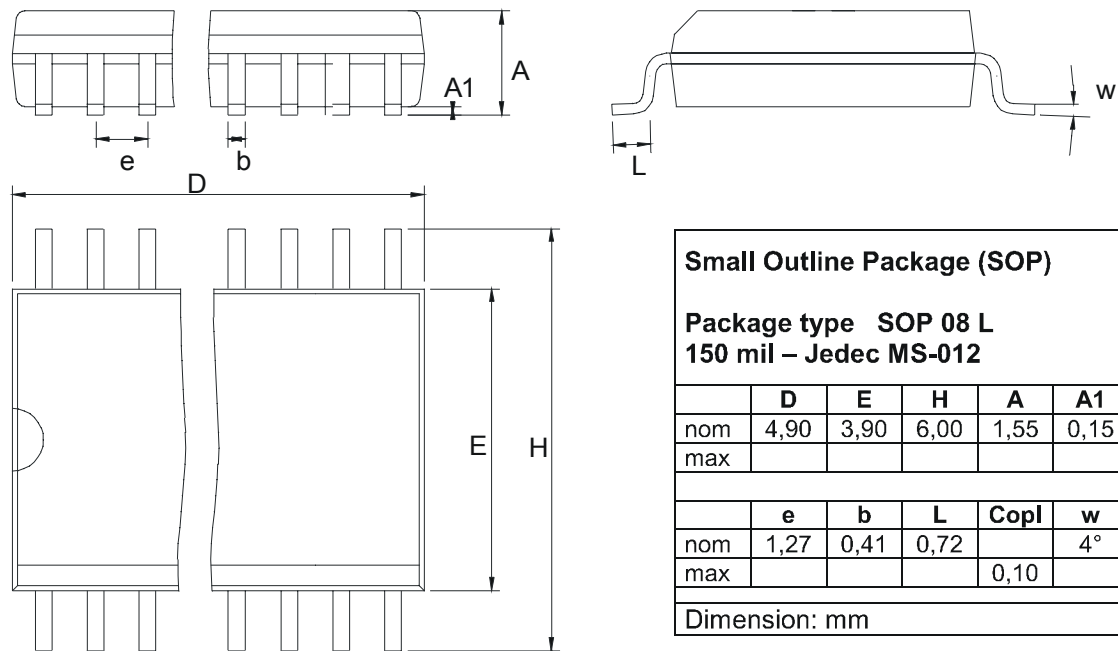
Figure 5: SOP 8 package dimensions
