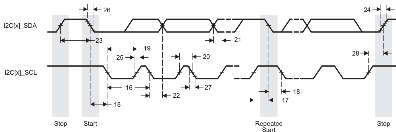
Figure 9-73. I2C Transmit Timing
