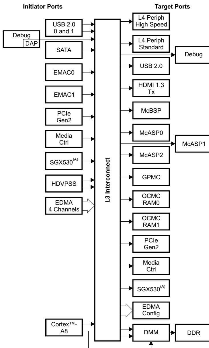
Figure 7-1. Interconnect Overview
