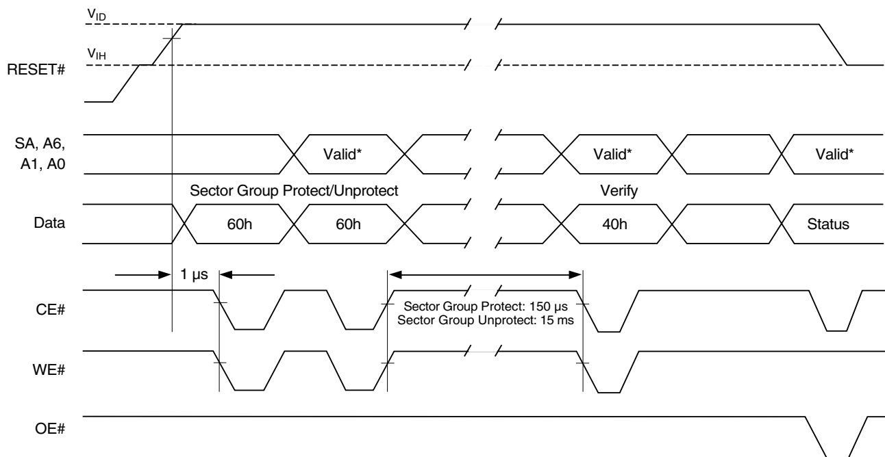
Figure 23. Sector/Sector Block Protect and Unprotect Timing Diagram
